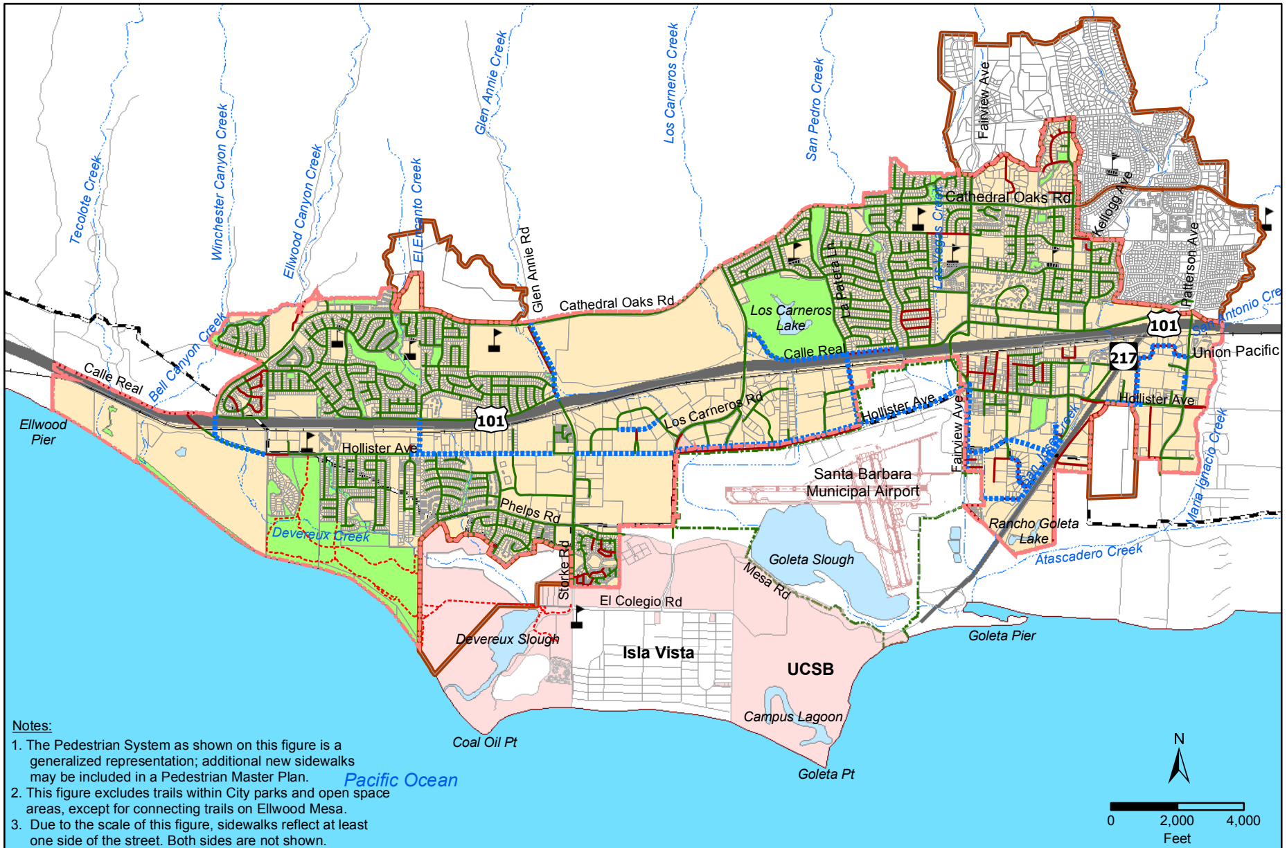
Figure 3.13-4 PEDESTRIAN SYSTEM PLAN
