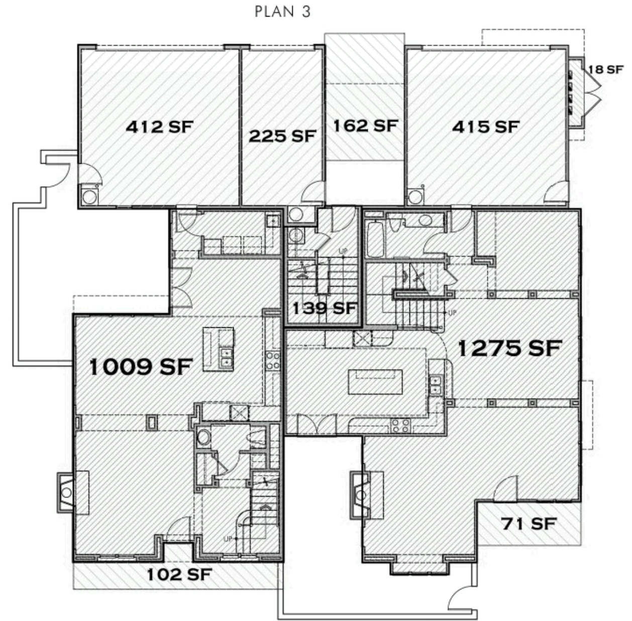
FIRST FLOOR
