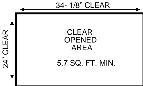
MINIMUM SIZE CLEAR OPENING FOR 24" CLEAR OPENED HEIGHT
