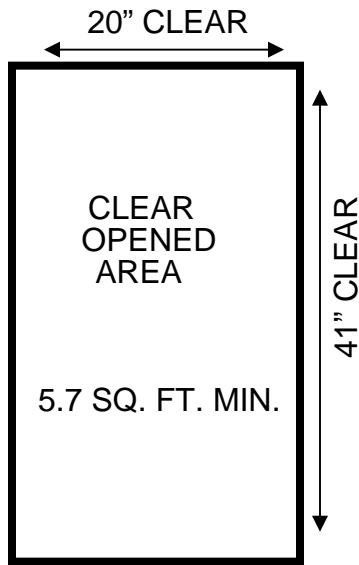
MINIMUM SIZE CLEAR OPENING FOR 20" CLEAR OPENED WIDTH
