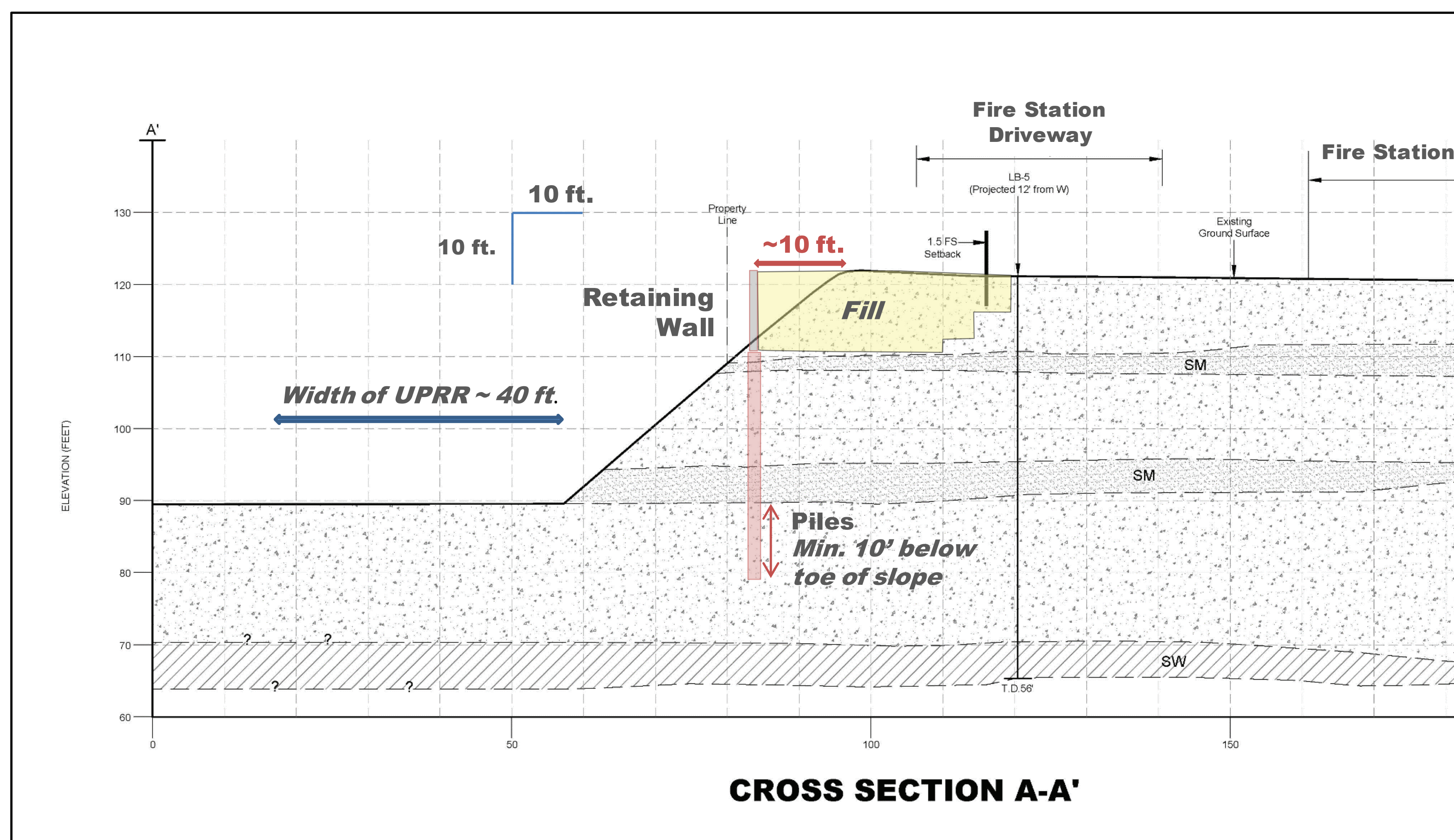
PROPOSED STABILIZATION - Deep Piles and Retaining Wall at/near property line
